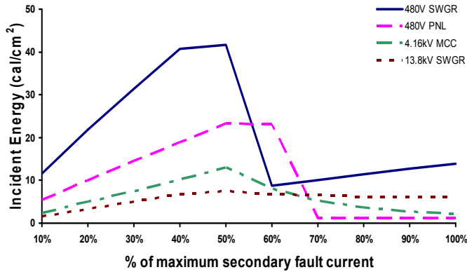
Fig. 5 Impact of fault current on incident energy calculations
