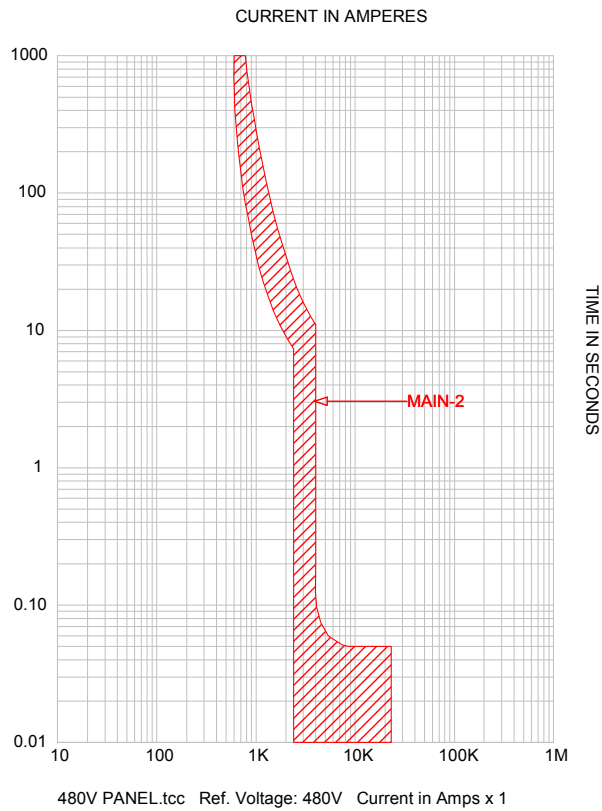
Fig. 4 Time Current Characteristics of the main protective devices in sample systems 1 through 4
