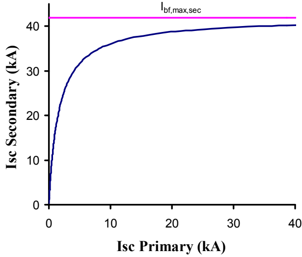
Fig. 2 Impact of changes in primary fault current to secondary fault current of a transformer
