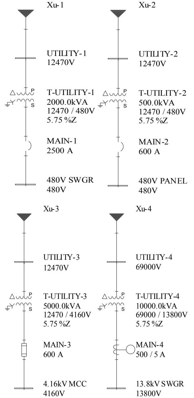
Fig. 3 Sample Systems 1, 2, 3 and 4
